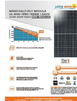
MONO HALF CUT 545~555 Watt
